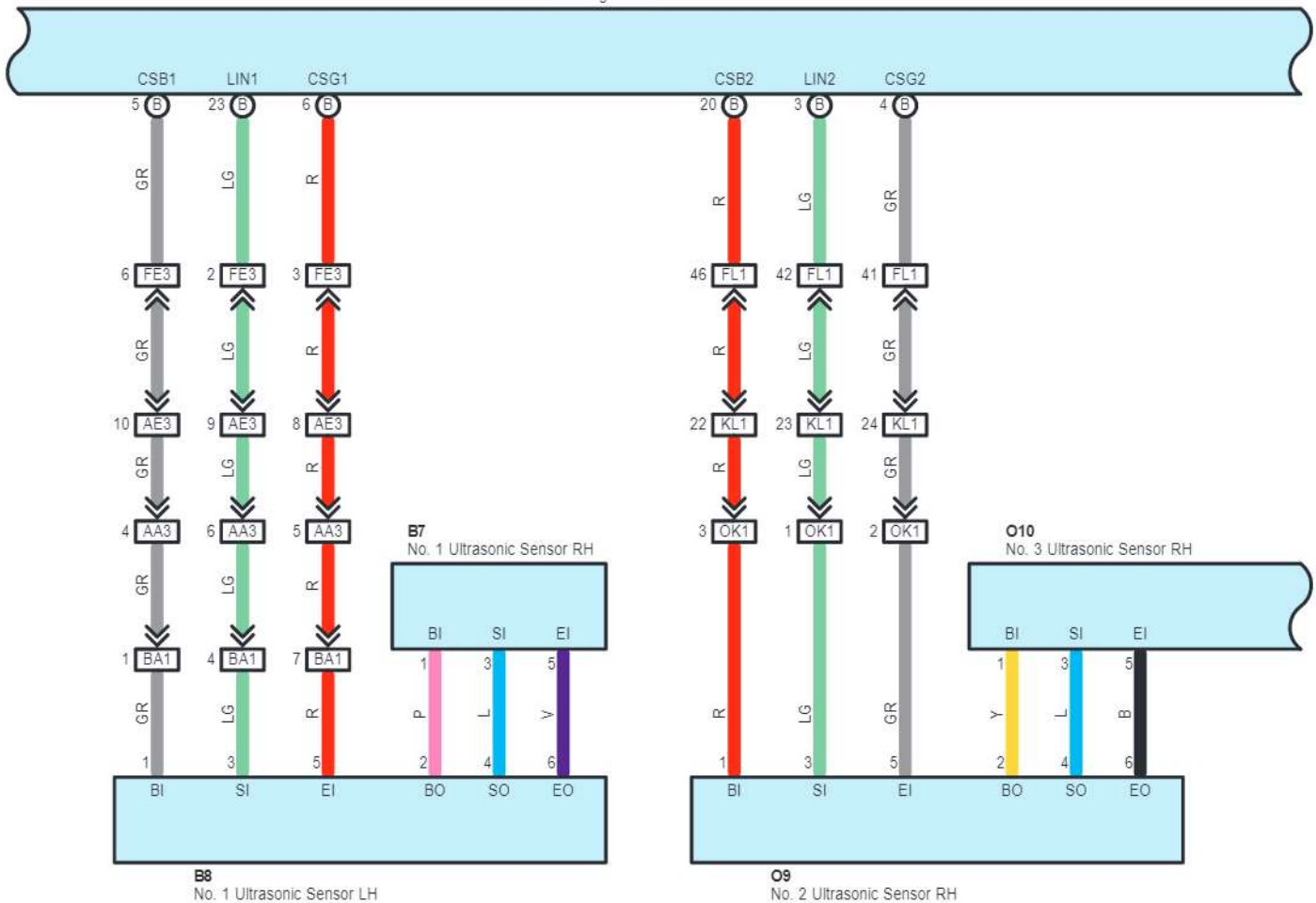
F75(A), F76(B), F81(C), F88(D) Parking Assist ECU
