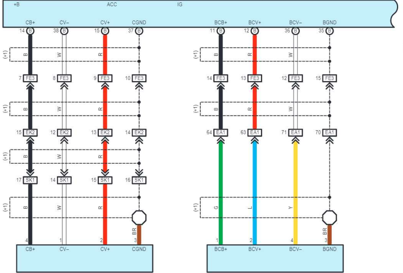
S5 Rear Television Camera Assembly
