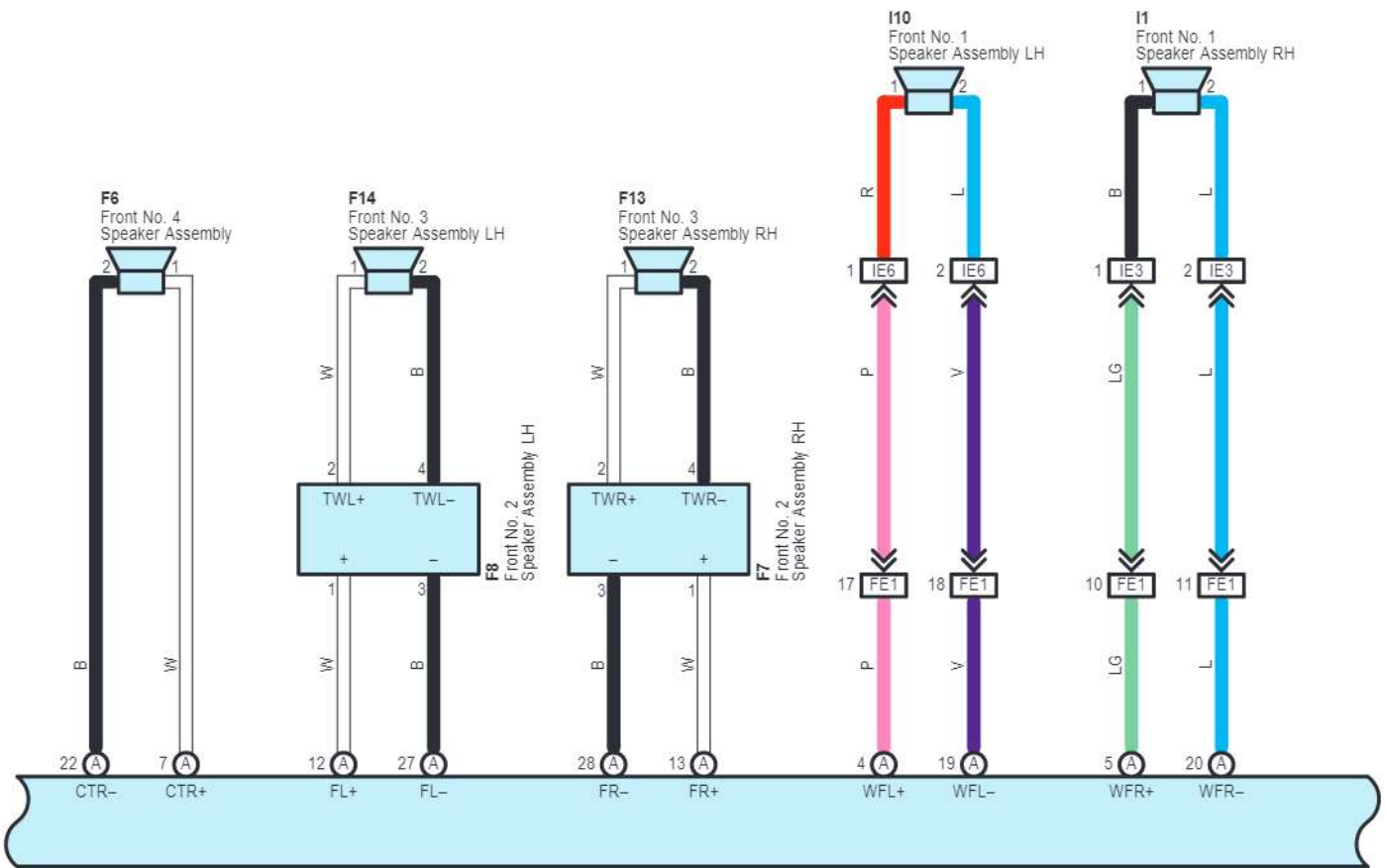
F74(A), F85(B) Stereo Component Amplifier Assembly
