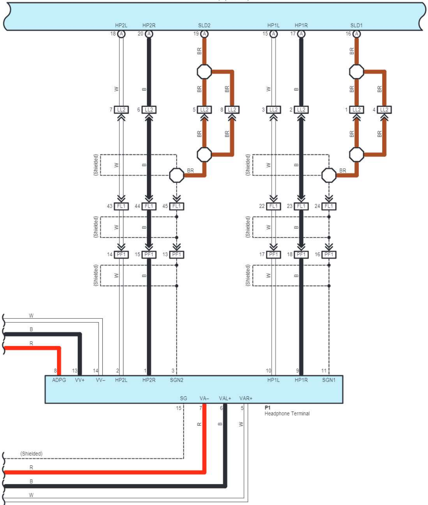
L39(A), L46(B) Television Display Assembly
